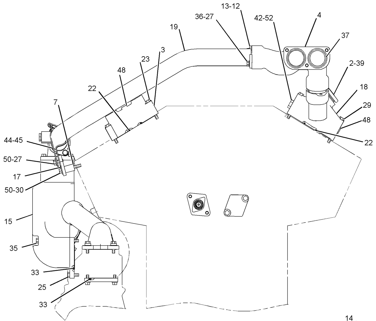
FRONT VIEW
