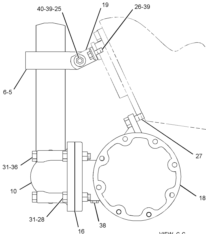
VIEW C-C
