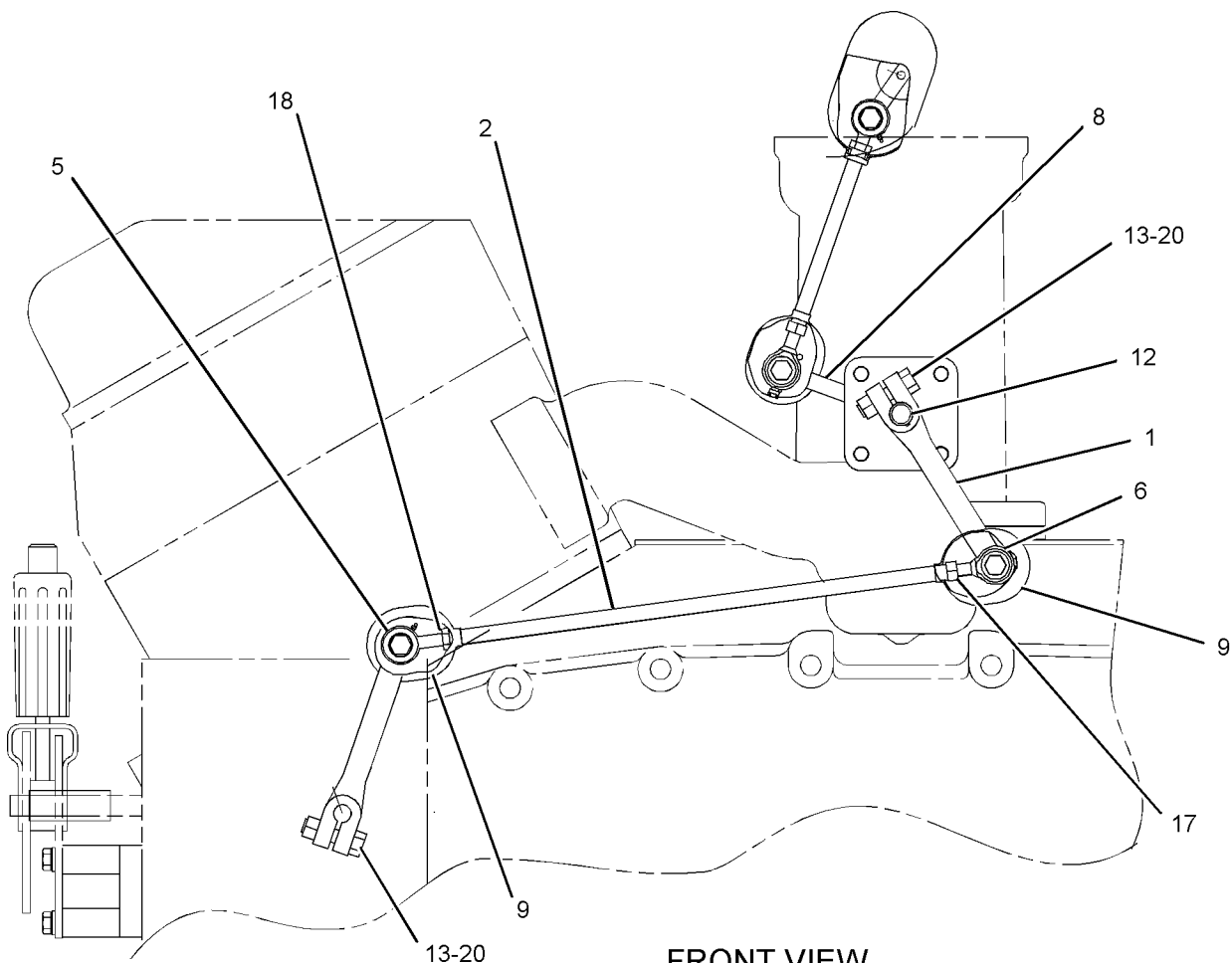
FRONT VIEW
