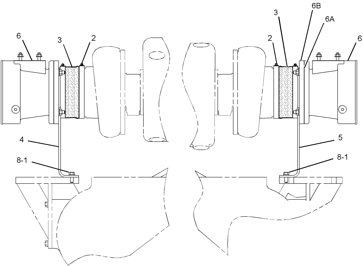
REAR VIEW
