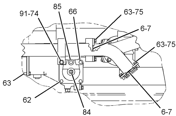
VIEW K-K
