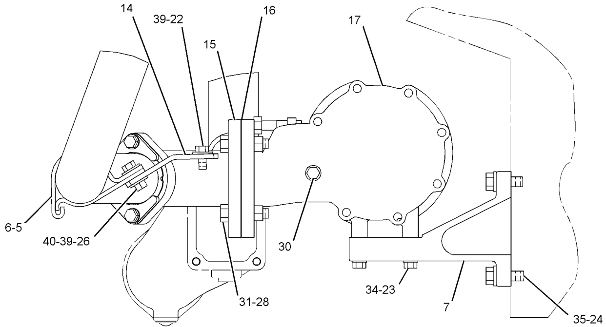
VIEW D-D
