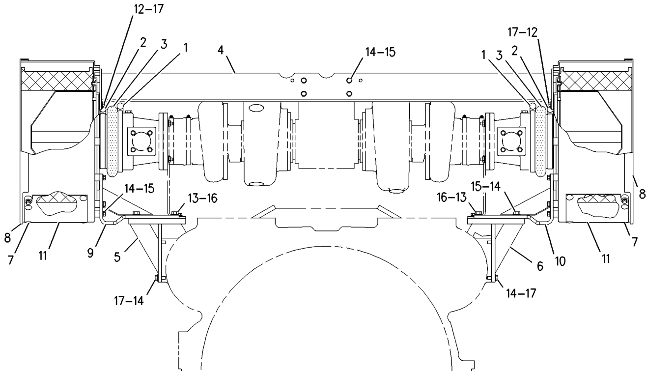
REAR VIEW
