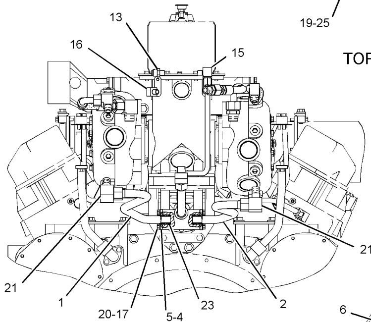
REAR VIEW OF ENGINE
