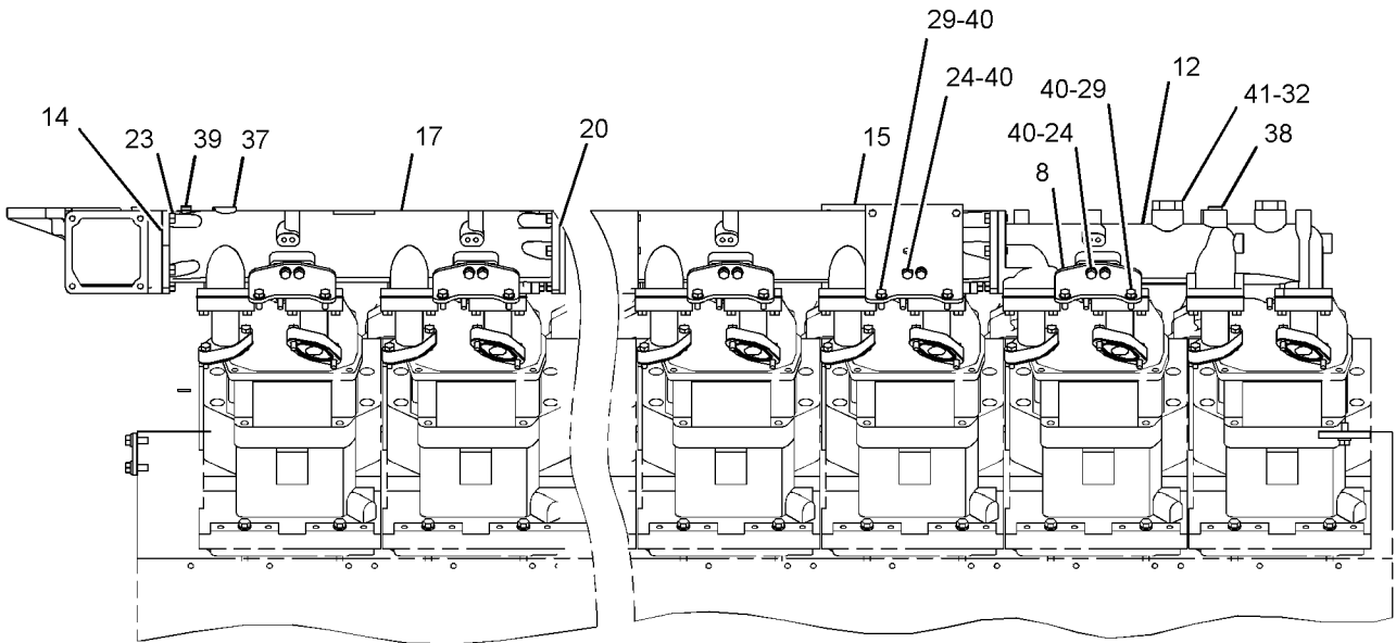
LEFT SIDE VIEW OF ENGINE
