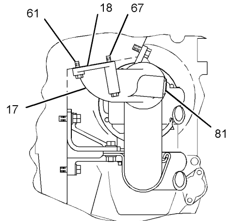
VIEW L-L
