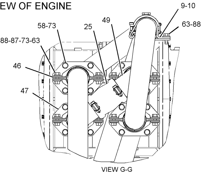
VIEW G-G
