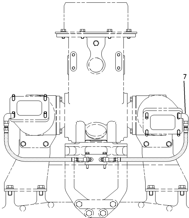
REAR VIEW
