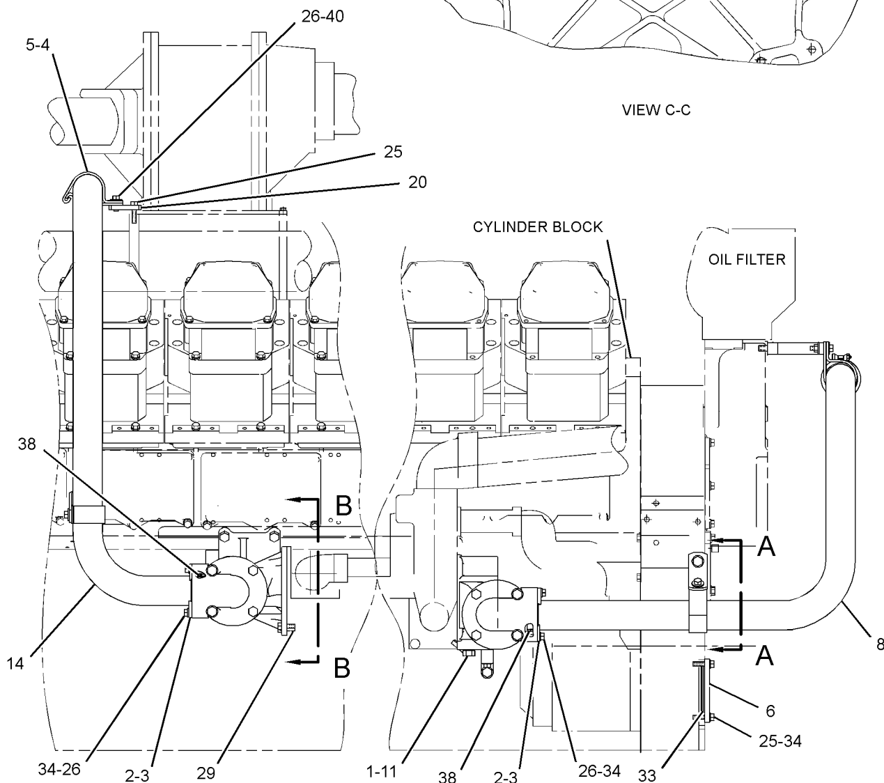
RIGHT SIDE VIEW OF ENGINE
