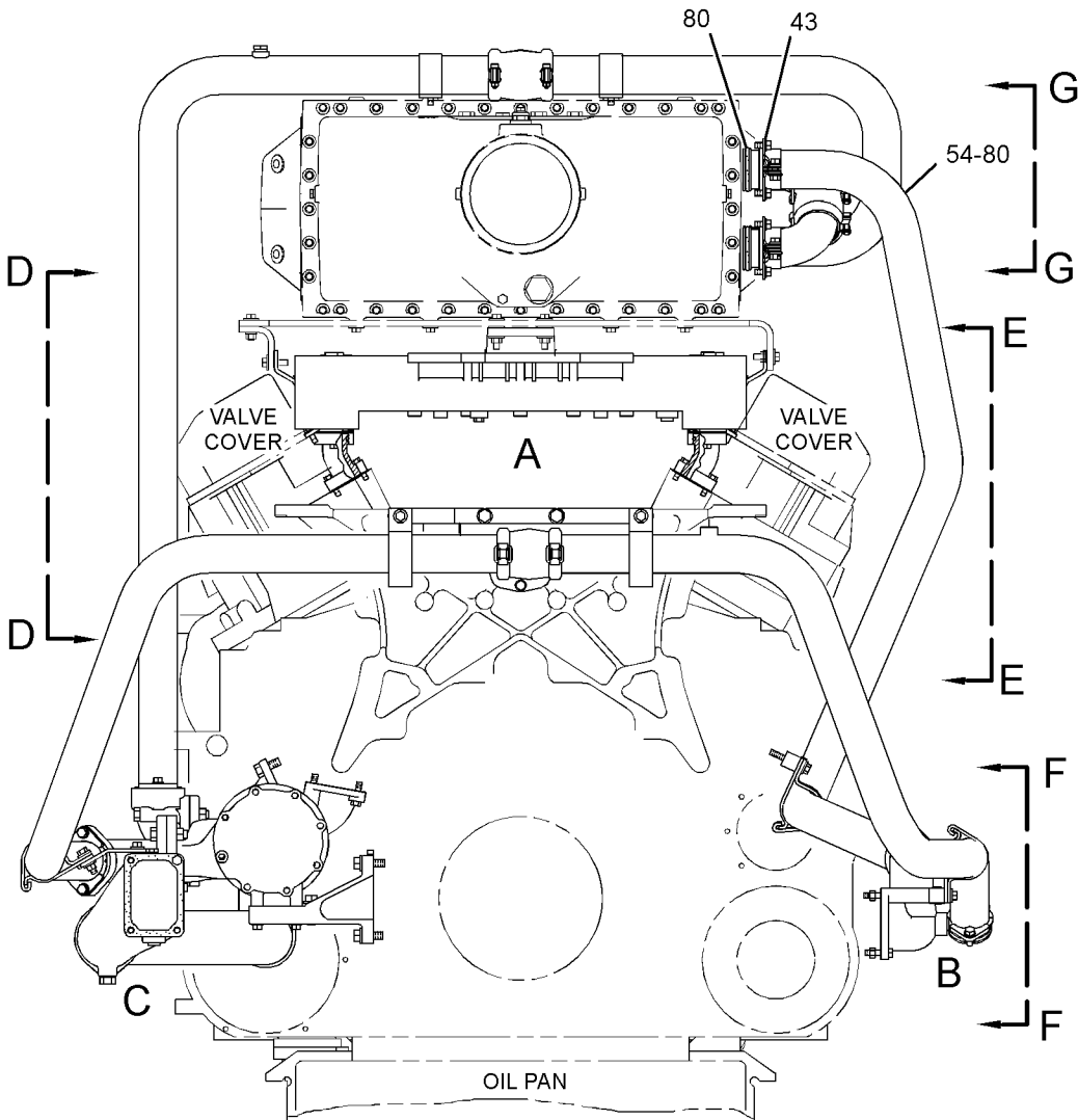
FRONT VIEW OF ENGINE
