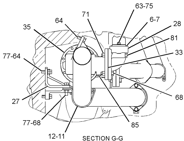
SECTION G-G
