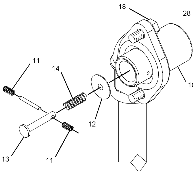
EXPLODED VIEW OF AREA B
