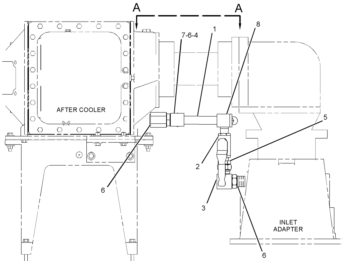
FRONT VIEW
