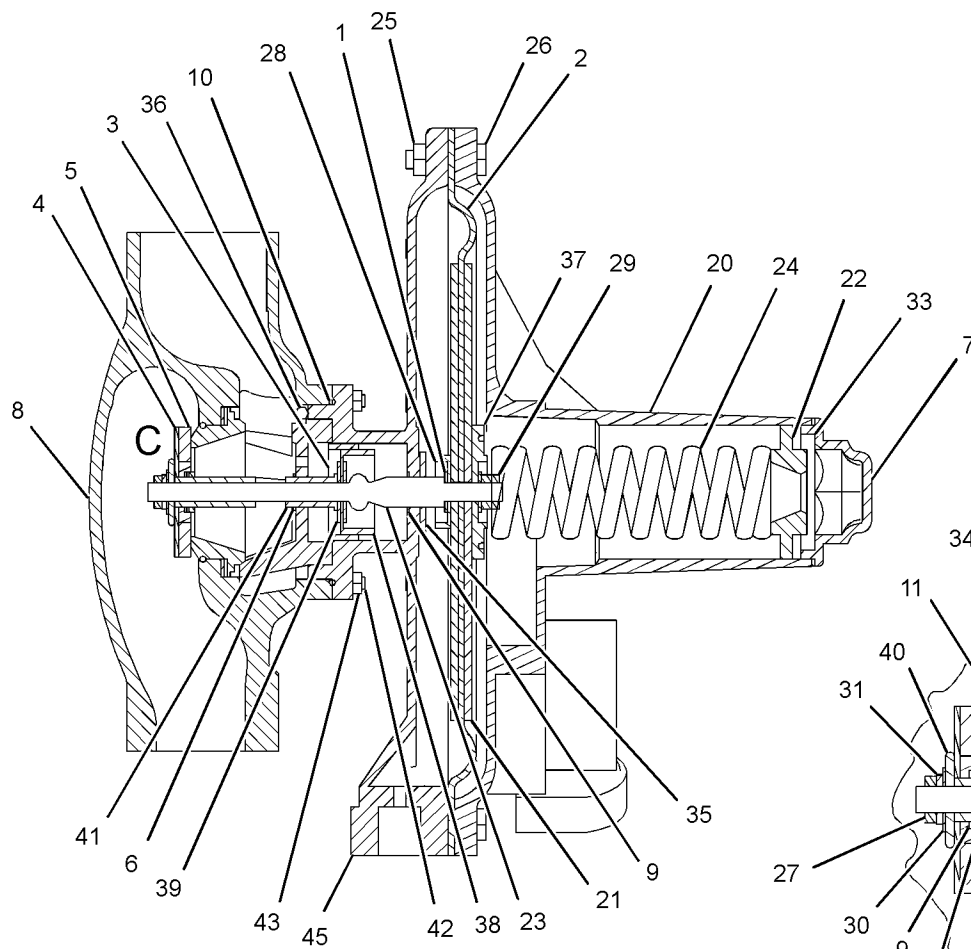
SECTION B-B
