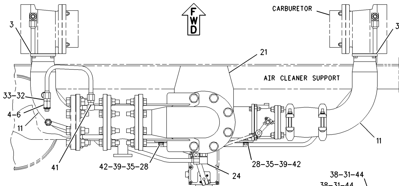
TOP VIEW
