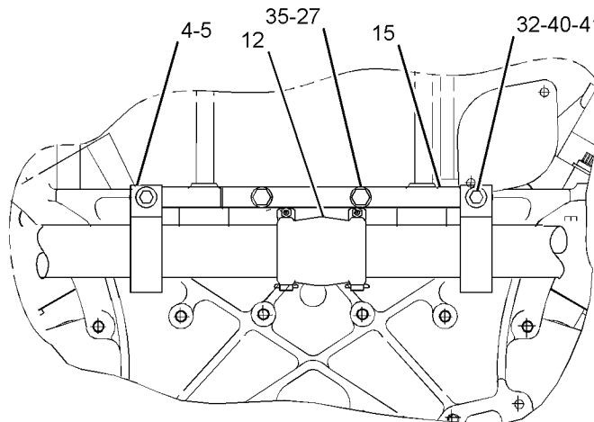
VIEW C-C
