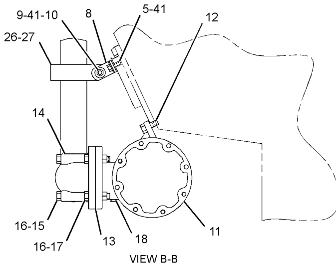
VIEW B-B
