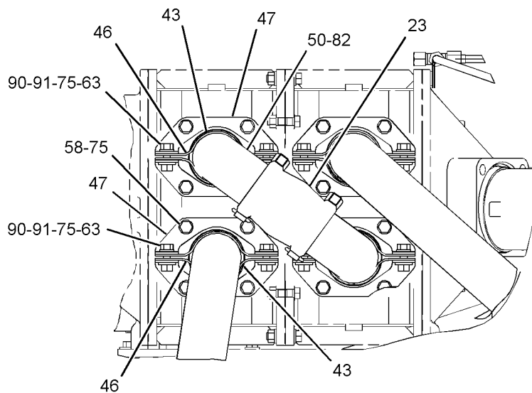
VIEW J-J
