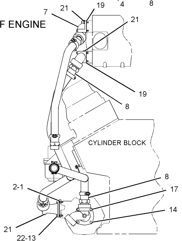
REAR VIEW OF ENGINE
