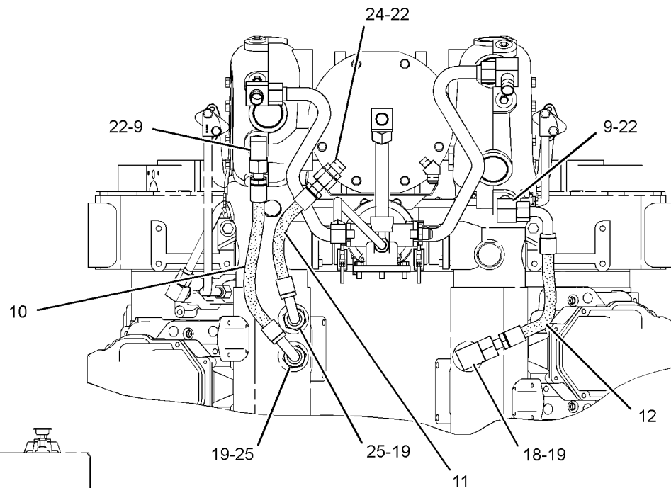
TOP VIEW OF ENGINE
