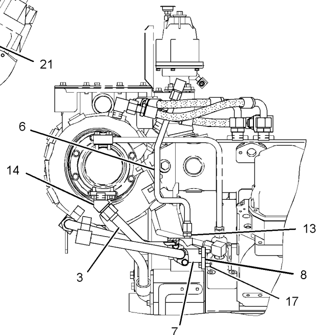
RIGHT SIDE VIEW OF ENGINE
