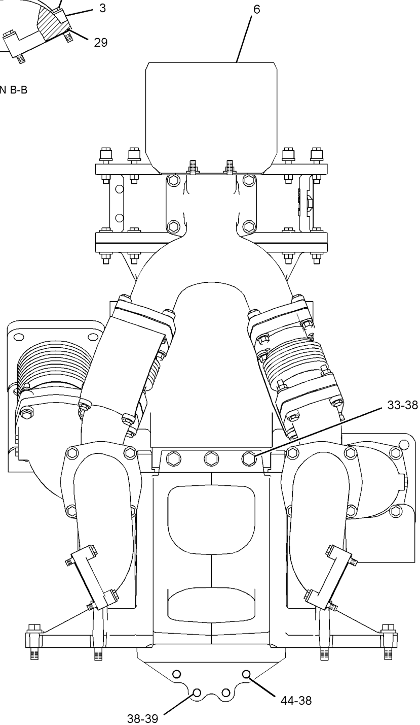
FRONT VIEW OF ENGINE
