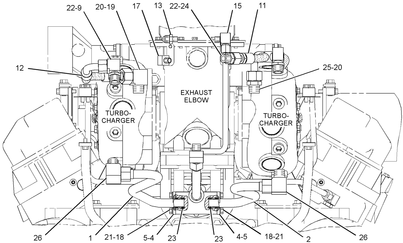
REAR VIEW OF ENGINE
