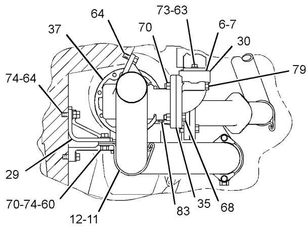
SECTION M-M
