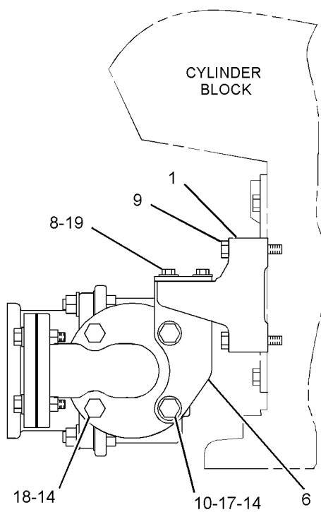
REAR VIEW OF ENGINE
