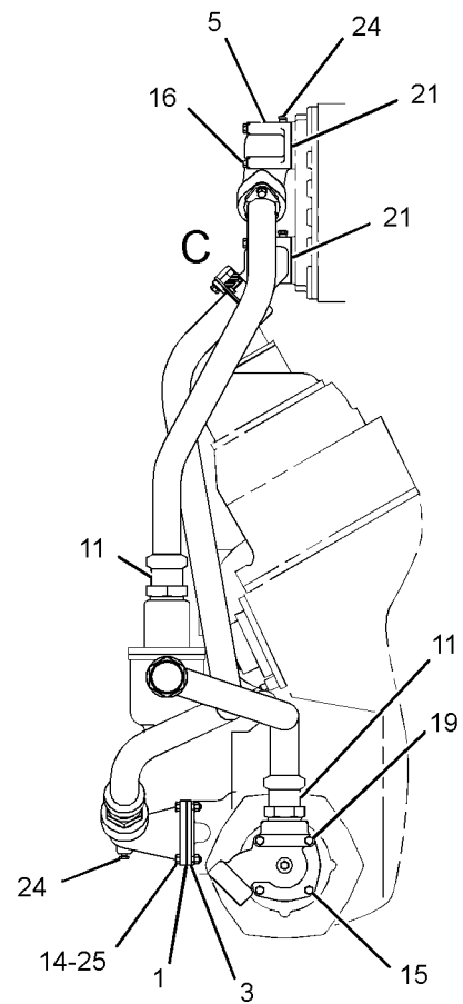
REAR VIEW
