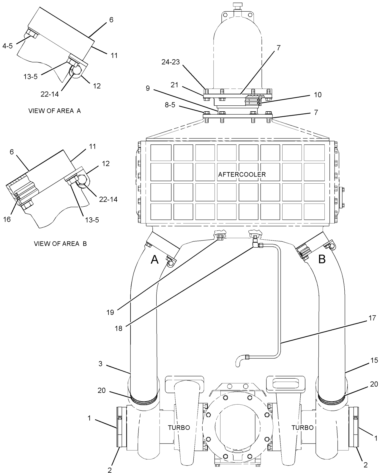
TOP VIEW OF ENGINE
