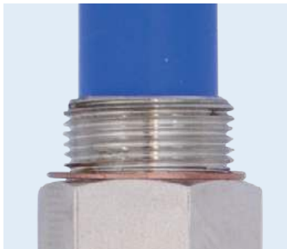
13/16-20 UNEF top thread for coil connection with full 6 threads to meet the CSA requirements
